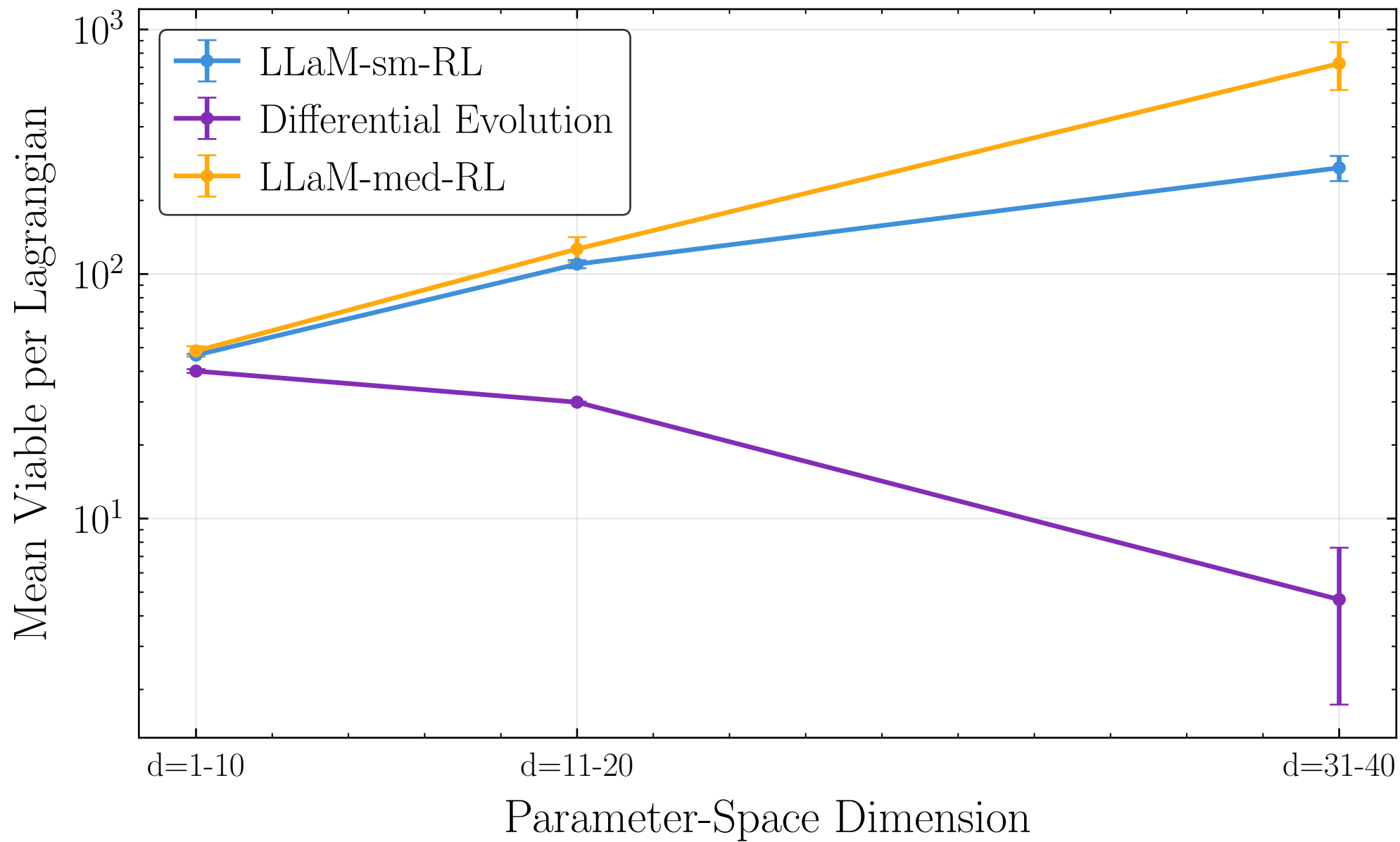
Mean Viable per Lagrangian vs Parameter-Space Dimension
