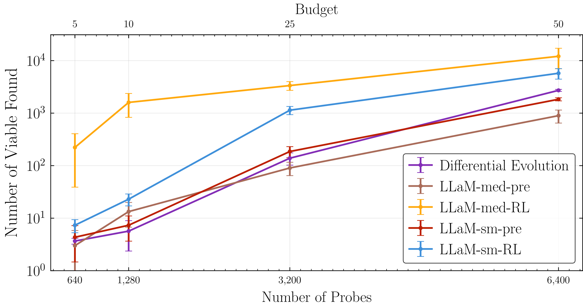
Total Viable Count vs Budget, summed over 21 Benchmark Lagrangians
